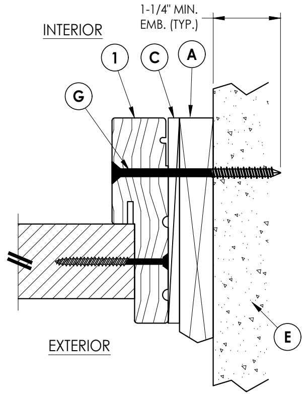
7 HORIZONTAL CROSS SECTION 2 Outswing 1X Buck Construction
